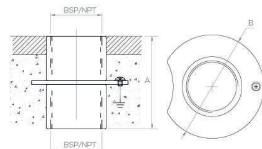
IF Model Female-Female Floor/Wall Fitting
